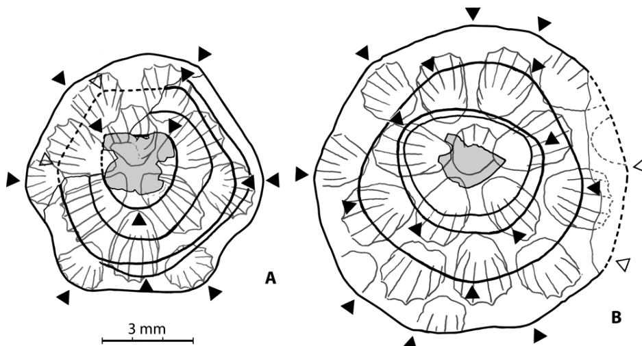
◀ Figure 2: Pinacopora ballica n. sp. Proximal side showing the main growth lines. The rounded angles ( i.e. , maximum curvature of the growth lines) giving rise to the successive polygonal outlines of the corallum are indicated by black triangles. Bioclast to which the larva was attached in grey. The upper surface (drawing of the natural mould) is seen in "transparency". A , specimen RGM 1 333 568 (see also Fig. 3.A). B , specimen RGM 1 333 571 (see also Fig. 3.E, .G).
