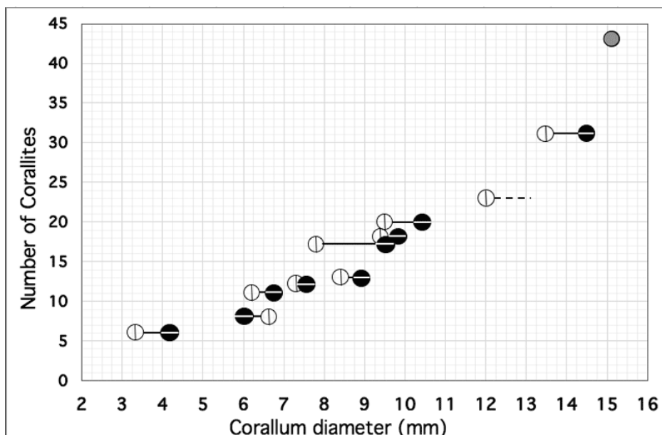
◀ Figure 8: Pinacopora bal-tica n. sp. Relationship between corallum diameter and number of corallites. Open circle with vertical bar as diameter in the plane of bilateral symmetry, black circle with horizontal bar as diameter normal to this plane and grey circle as average diameter of the largest specimen. This specimen (RGM 1 333 578) is somewhat deformed nearly the plane of bilateral symmetry of the colony and thus the two above diameter are not available with sufficient confidence, it is why only an apparent average (15.1) between maximum (16.0) and minimum (14.2) diameter is used. Some data, diameter or number of corallites, are estimated (see Table 1). Specimen with silicified skeleton (RGM 1 333 577) too incomplete, not taken into account.
